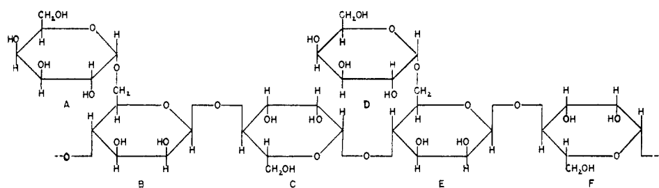
Section of guarán molecule.
